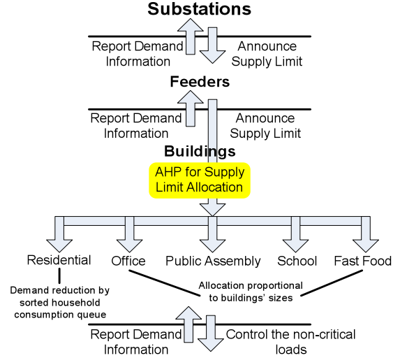
Fig. 6. Multi-layer DR structure.
